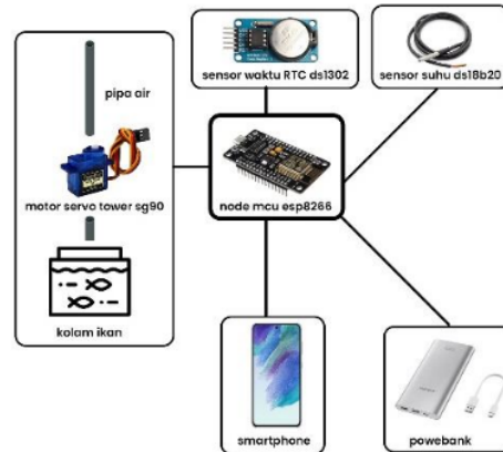
Figure 2. Hardware Suite and Web Apps Source: Observation results, 2022
